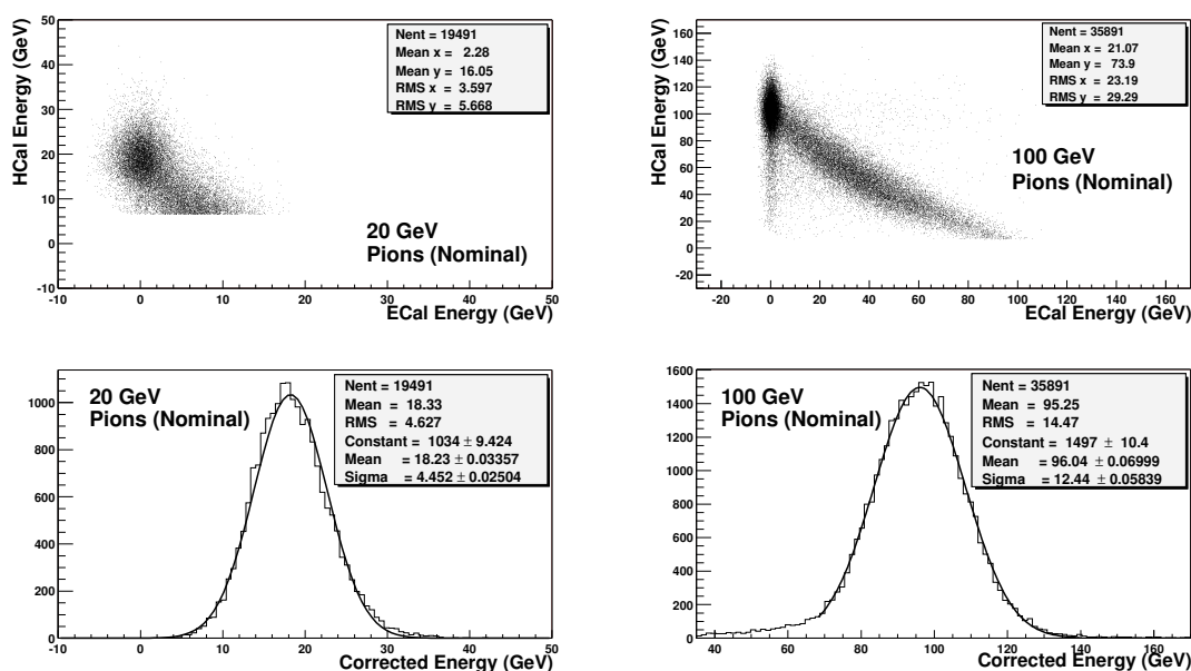
Figure 5.25: Energy distributions of 20 GeV and 100 GeV pions, after the HCAL versus ECAL energy based background cuts were applied. Some signal events are lost at low energies. The non-Gaussian low energy tails are due to energy leakage beyond the HB outer limits.
