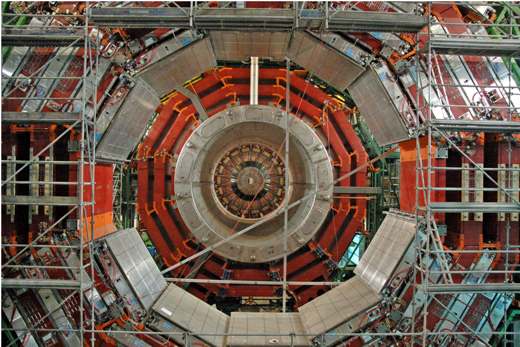
Figure CP 3: View along the axis of the completed CMS magnet, showing also installed DT chambers, CSCs, and HE.
