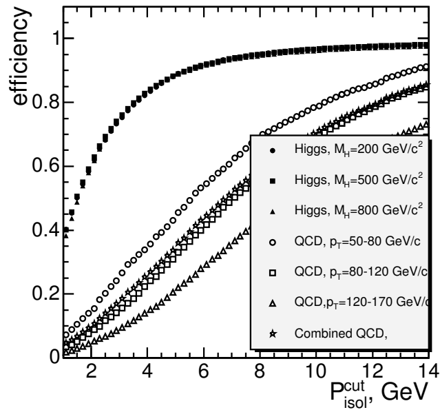
Figure 12.19: The efficiency of the ECAL isolation in the High Level Trigger for the signal and the QCD multi-jet background as a function of the cut P_{\text{isol}}^{\text{cut}} on the ECAL isolation parameter.
