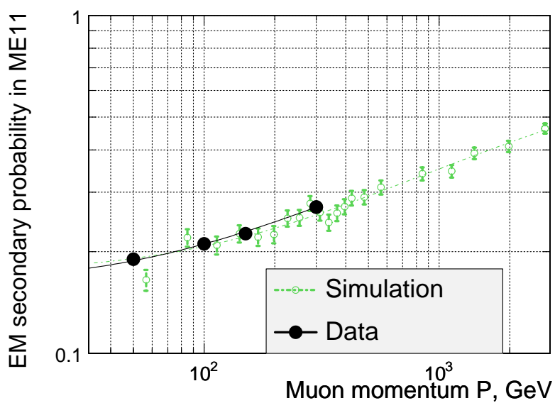
Figure 3.18: Electromagnetic secondaries probability in ME1/1 vs muon beam energy.
