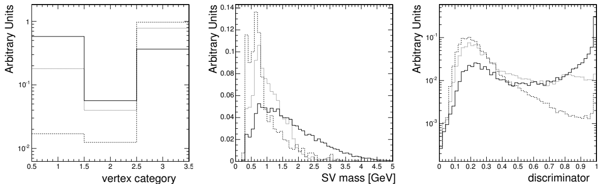
Figure 12.27: Distribution of the vertex category (left), reconstructed secondary vertex mass (middle) and combined discriminator (right) for b -jets (solid), c -jets (dotted) and uds -jets (dashed, udsg -jets for the rightmost plot) as obtained from a sample of QCD events for jets with underlying parton momenta between 50 and 80 \text{GeV}/c .
