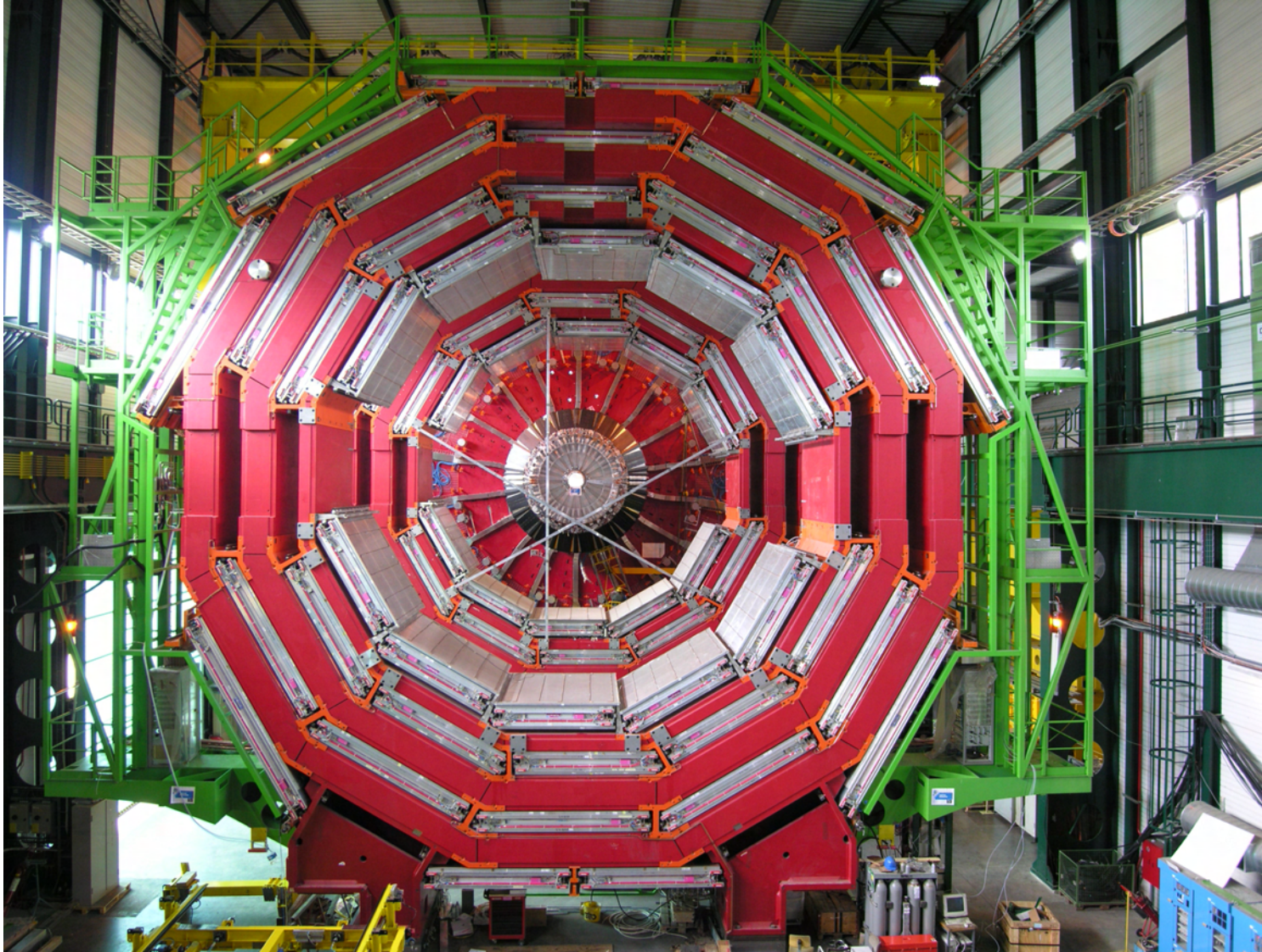
Figure CP 4: Installation of DT chambers into the YB+1 wheel.
