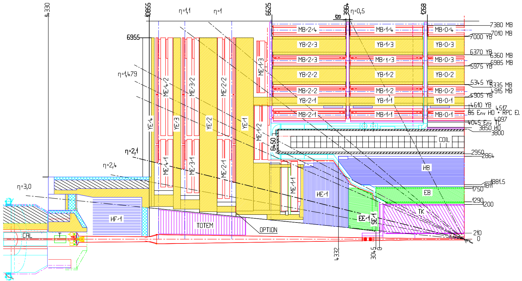
Figure CP 1: One quarter longitudinal view of the CMS Experiment. Dimensions are in units of mm.
