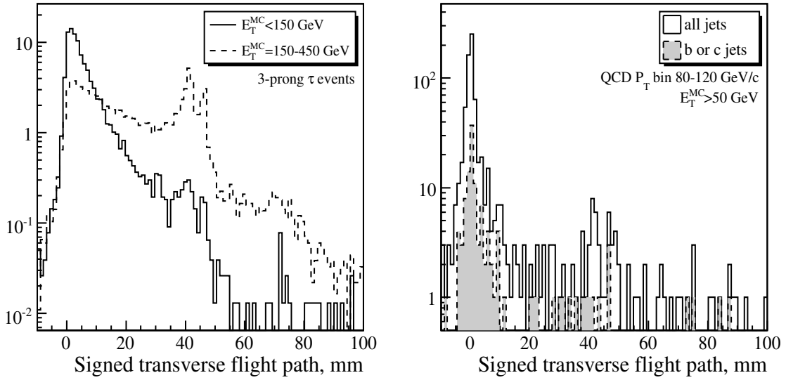
Figure 12.12: The signed transverse flight path for \tau (left) and QCD (right) jets passing the tracker isolation requirement. Three reconstructed tracks are required to be in the signal cone. See text for more details.
