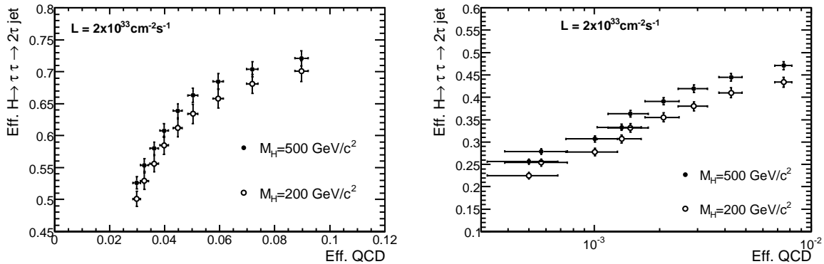
Figure 12.20: Efficiency of Calo+Px1 trigger applied to the first jet (left plot) and to both jets (right plot) for signal events versus efficiency for QCD multi-jet events. Two Higgs boson masses of M_H=200 and 500 \text{ GeV}/c^2 are shown. The isolation cone is varied from 0.2 to 0.6 in steps of 0.05; the signal cone is 0.07; the matching cone is 0.1; and the p_T of the leading tracks must exceed 3 \text{ GeV}/c .
