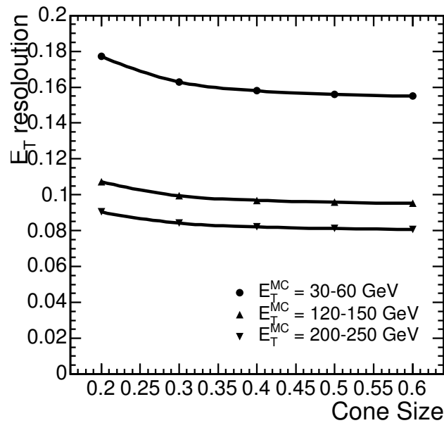
Figure 12.2: The transverse energy resolution of \tau jet as a function of the reconstructed cone size for the different bins of E_T^{\text{MC}} .
