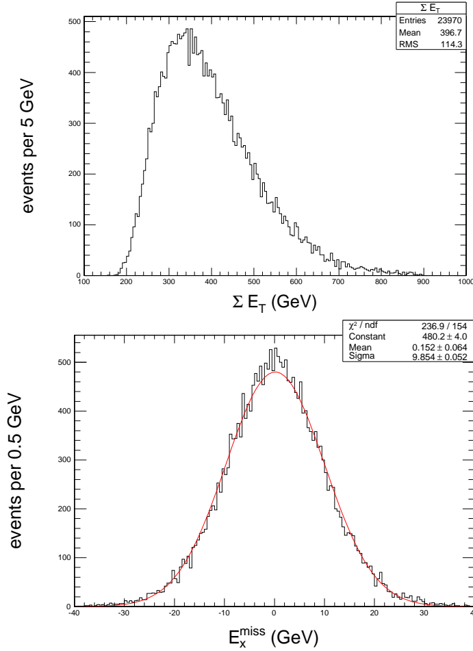
Figure 11.11: Top) Distribution of \Sigma E_T and Bottom) E_x^{\text{miss}} for soft QCD events ( 0 < \hat{p}_T < 15 \text{ GeV} ) with pile-up. The resolution is 9.9 GeV in agreement with expectations based the study with minimum bias events.
