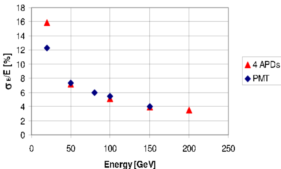
Figure 7.15: Comparison of the energy resolution with the PMT and 4 APDs as the readout.
