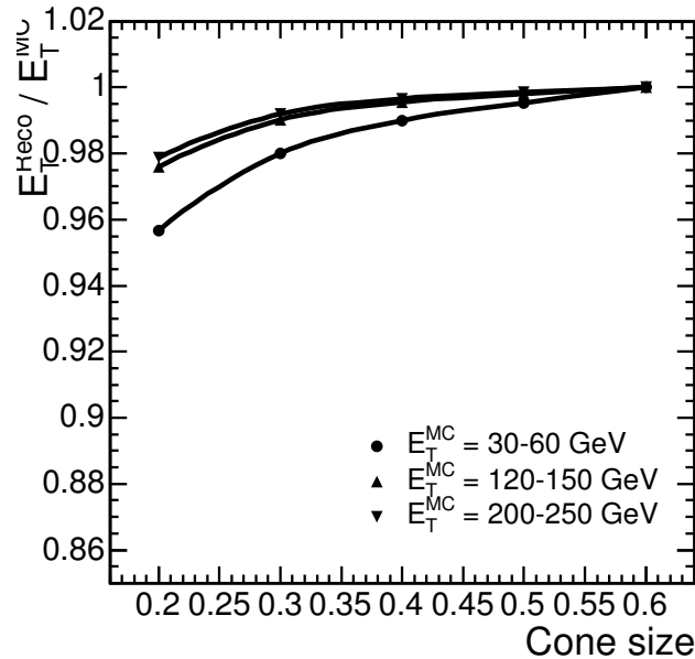
Figure 12.1: The ratio r = E_T^{\text{reco}} / E_T^{\text{MC}} as a function of the reconstruction cone size for different bins of E_T^{\text{MC}} . The values of r were normalized to unity at a cone size of 0.6.
