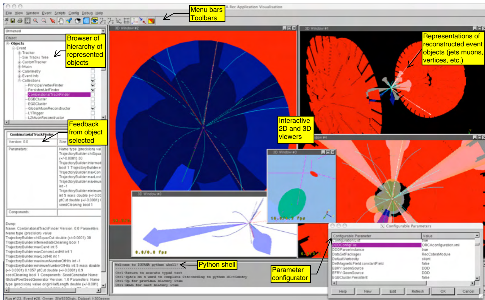
Figure CP 14: Screen shot of the interactive IGUANA-based CMS detector and event display, showing reconstructed objects such as tracks, jets, and vertices in 2D and 3D views.
