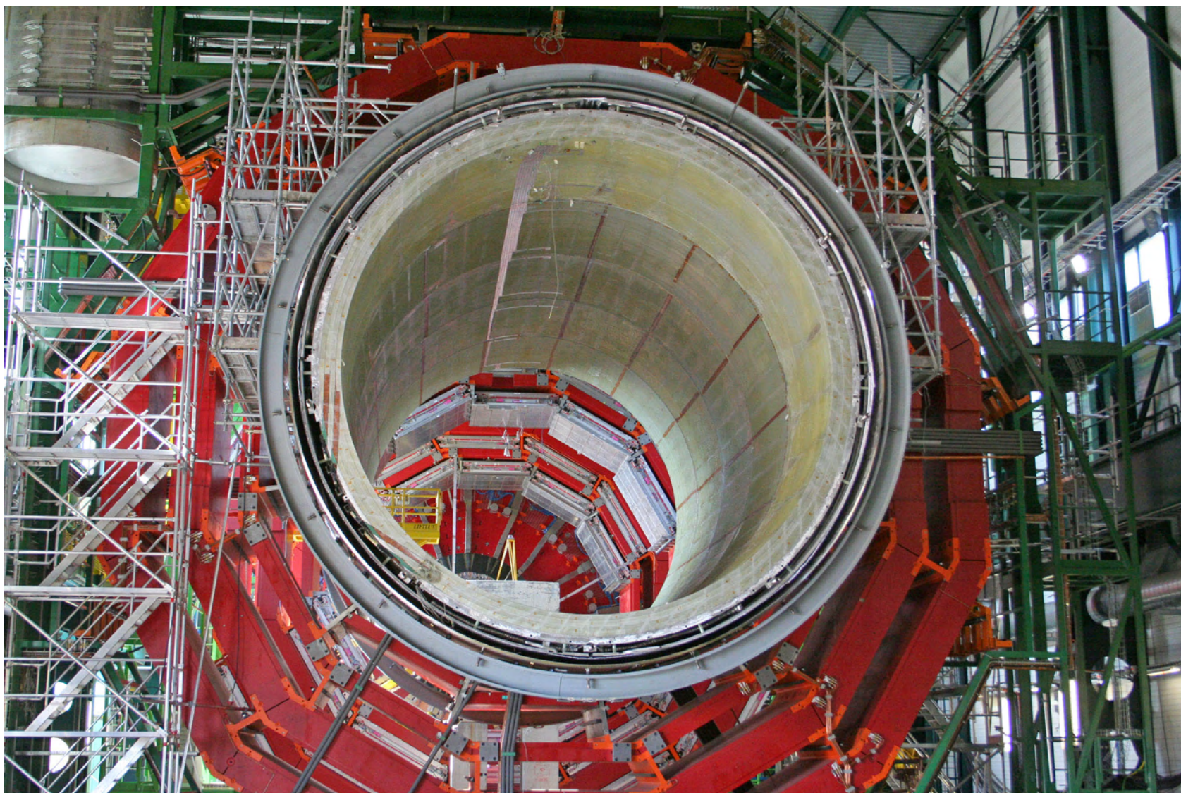
Figure CP 2: Assembly of the yoke of the CMS magnet. The outer vacuum tank and the coil can be seen.
