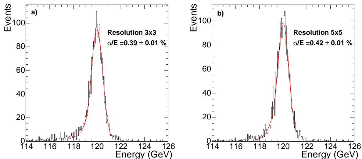
Figure 4.12: Distribution of the energy reconstructed in (a) a 3 \times 3 cluster and (b) a 5 \times 5 cluster, when 120 GeV electrons are incident in a 4 \times 4 \text{ mm}^2 region.
