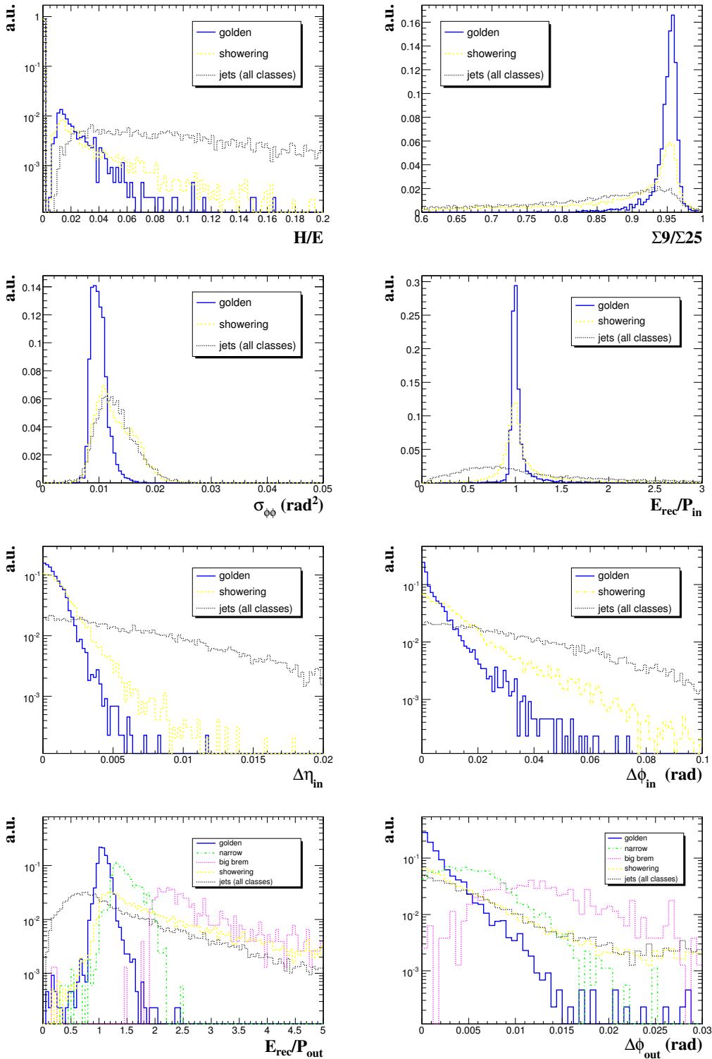
Figure 10.29: Distributions of electron identification observables in the \eta range of the ECAL barrel . The distributions of shower shape and track-supercluster matching observables are shown for different classes of electrons. Electrons uniformly distributed in p_T^e between 5 and 50 GeV/c are compared to "fake" electron candidates found in jets from a QCD di-jet background generated in the range 25 < \hat{p}_T < 170 GeV/c.
