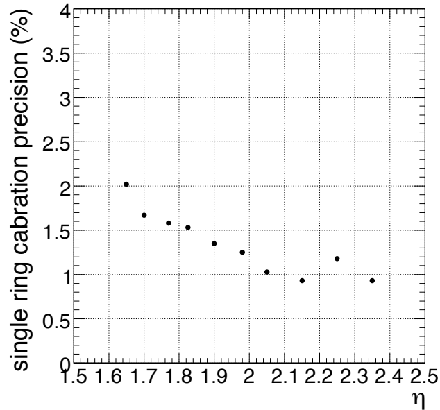
Figure 4.22: Calibration precision versus \eta for 7 \text{ fb}^{-1} of integrated luminosity.
