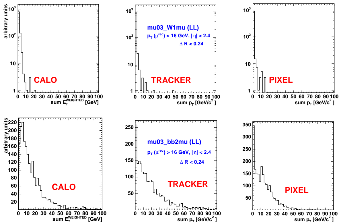
Figure 9.26: Distributions of the energy deposited in a \Delta R = 0.24 isolation cone for the calorimeter (left), the full tracker (centre), and the pixel tracker only (right). The difference in energy deposits between a typical source of isolated muons ( W \rightarrow \mu X , top) and non-isolated muons ( b\bar{b} \rightarrow 2\mu X , bottom) is well visible. The distributions are for the low-luminosity case.
