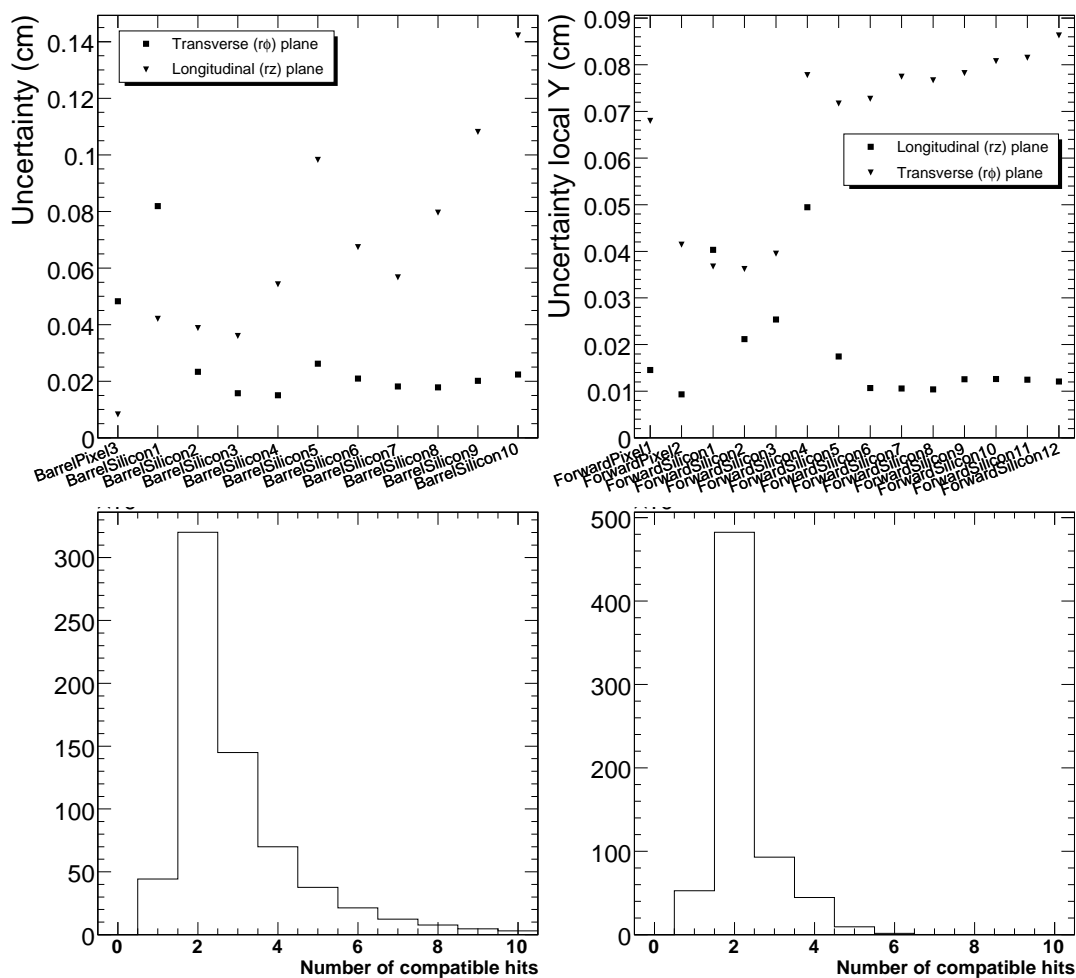
Figure 6.13: Upper figures: Mean uncertainties of the predicted state in the barrel (left) and forward tracker (right) in the transverse ( r\text{-}\phi ) and longitudinal ( r\text{-}z ) planes. Lower figures: number of compatible hits (including invalid hit(s)) found per trajectory, when leaving the pixel barrel layer 3 (left) and TIB layer 3 (right). Simulated b -jets with transverse momenta between 120 and 170 GeV/ c are used, with low luminosity pile-up included.
