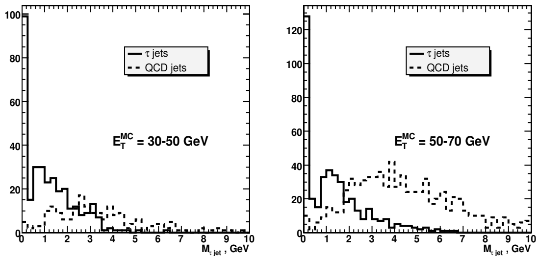
Figure 12.16: The M_{\tau \text{ jet}} distributions for \tau jets (solid line) and QCD jets (dashed line) in the E_{\tau}^{\text{MC}} bins of 30–50 GeV (left plot) and 50–70 GeV (right plot).
