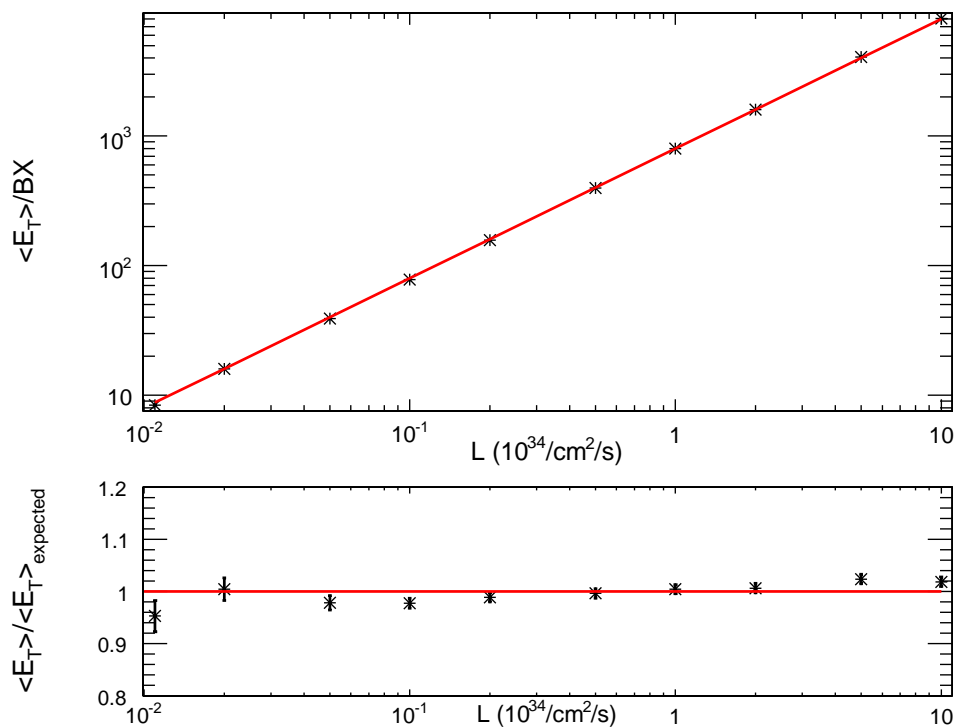
Figure 8.4: Linearity test of the HF E_T sum technique. The upper panel shows the average E_T per bunch crossing vs. the luminosity expressed in units of the LHC design luminosity of \mathcal{L} = 10^{34} \text{ cm}^{-2} \text{ s}^{-1} . The lower panel shows the same data plotted relative to what is expected for a linear response. See text for additional details.
