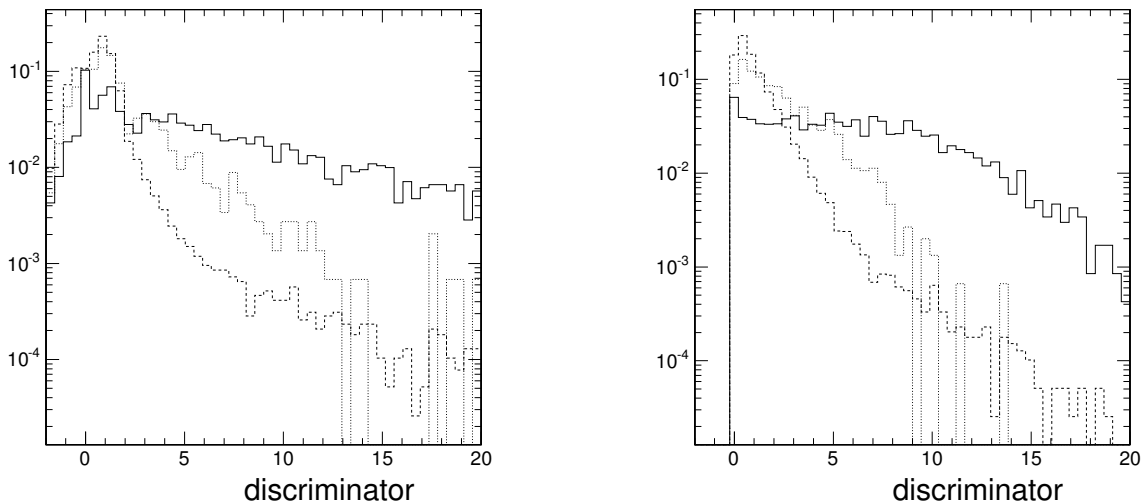
Figure 12.26: Distribution of the discriminator for the track counting algorithm ( N = 2 ) (left) and the track probability algorithm (right) for b -jets (solid), c -jets (dotted) and udsq -jets (dashed).
