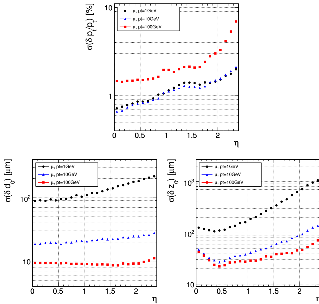
Figure 1.11: Resolution of several track parameters for single muons with transverse momenta of 1, 10 and 100 GeV/ c : (upper) transverse momentum, (lower left) transverse impact parameter, and (lower right) longitudinal impact parameter.
