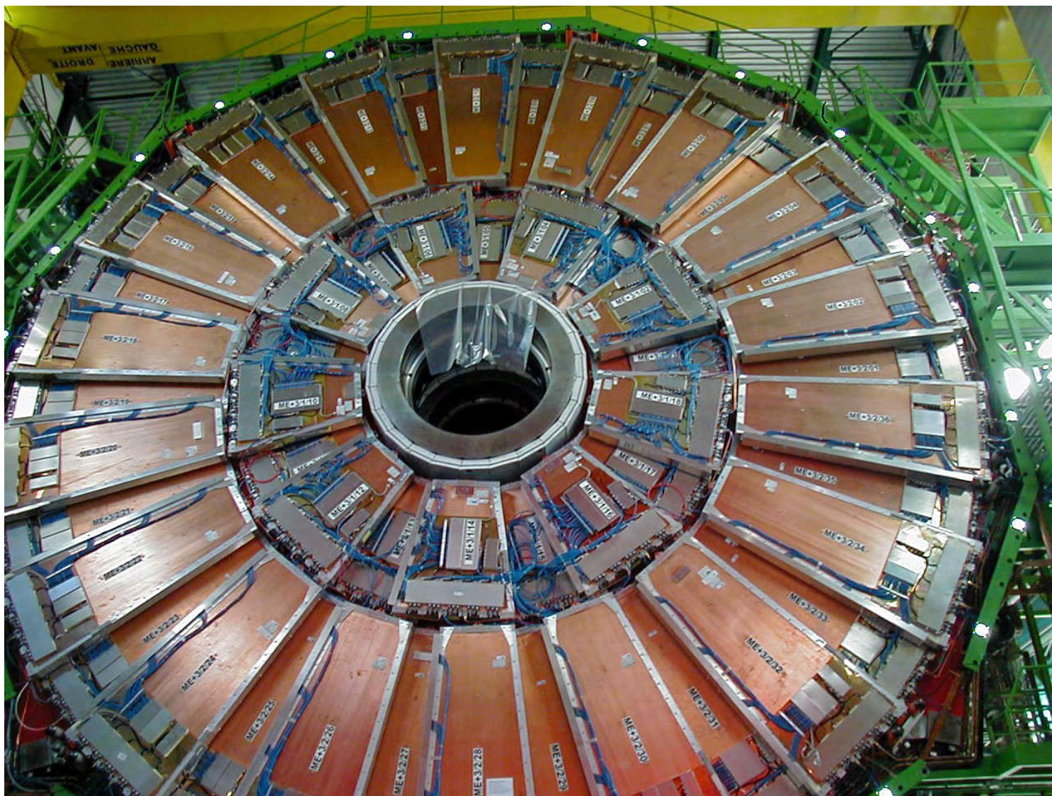
Figure CP 5: Installation of CSC chambers onto the YE+2 disk.
