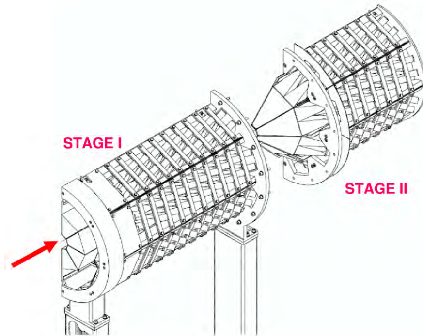
Figure 7.4: View of the mechanical design of the calorimeter showing the 2 stages.
