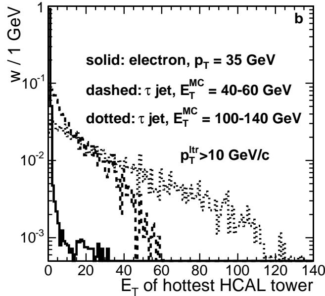
Figure 12.18: The transverse energy of the hottest (maximal E_T ) HCAL tower belonging to the reconstructed jet. Solid line—electron of p_T = 35 GeV/ c reconstructed as a jet. Dashed (dotted) line— \tau jet in the range true \tau -jet transverse energy of 40–60 GeV (100–140 GeV). A cut on the measured transverse momentum of the leading track in \tau jet, p_T^{\text{ltr}} > 10 GeV/ c , was applied. All histograms are normalized to unit area.
