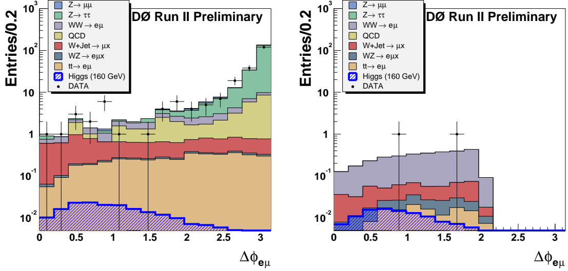
Figure 9: Difference in azimuthal angle of the reconstructed electron and muon at an early stage of the selection (left) and after all cuts (right) in the search for H \rightarrow WW \rightarrow e\nu\mu\nu in D\phi Run II data corresponding to an integrated luminosity of 176 \text{ pb}^{-1} (from Ref. 52).
