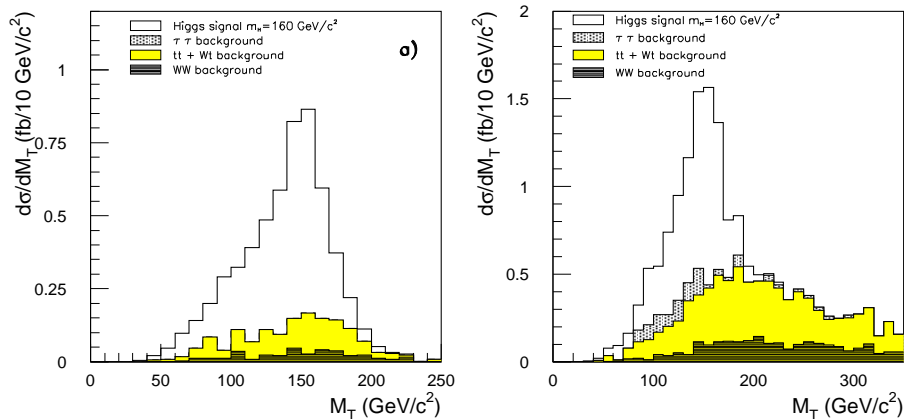
Figure 19: (Left) Distribution of the transverse mass M_T for a Higgs boson with a mass of 160 \text{ GeV}/c^2 and the backgrounds in the e\mu -channel after all cuts. (Right) The same, after relaxing kinematical cuts on the reconstructed leptons. The accepted cross sections d\sigma/dM_T (in \text{fb}/10 \text{ GeV}/c^2 ) including all efficiency and acceptance factors are shown in both cases (from Ref. 79).
