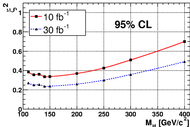
Figure 40: \xi^2 values (see text) which can be excluded with a confidence level of 95% for integrated luminosities of 10 and 30 fb -1 as a function of the Higgs boson mass (from Ref. 178).
