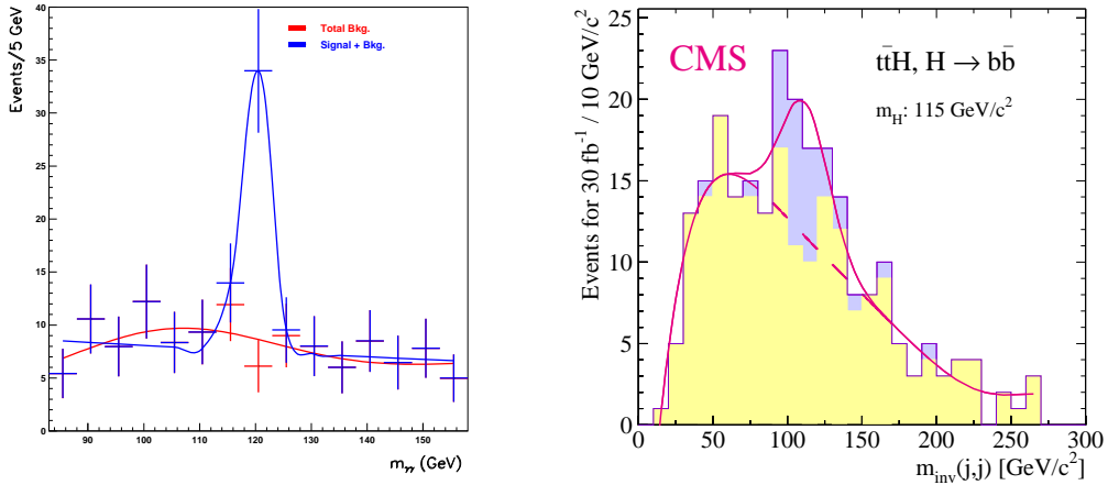
Figure 23: (Left) Reconstructed \gamma\gamma invariant mass distribution after the \gamma\gamma + \cancel{E}_T selection for an integrated luminosity of 100 \text{ fb}^{-1} (from Ref. 95). (Right) Reconstructed b\bar{b} invariant mass distribution of a t\bar{t}H \rightarrow \ell\nu b q\bar{q} b\bar{b} signal (dark) with m_H = 115 \text{ GeV}/c^2 and the background (light) for an integrated luminosity of 30 \text{ fb}^{-1} (from Ref. 100).
