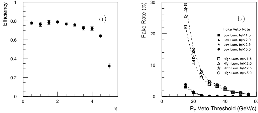
Figure 18: (Left) Efficiency for reconstructing a tag jet with P_T > 20 GeV/c which originates from a parton with P_T > 20 GeV/c as a function of pseudorapidity \eta of the parton. (Right) Probability for finding at least one jet from pile-up events in central rapidity intervals in the ATLAS detector as a function of jet P_T threshold. The dashed curves connect the points for pseudorapidity intervals |\eta| < 1.5 and |\eta| < 3.0 for low and high LHC luminosities.
