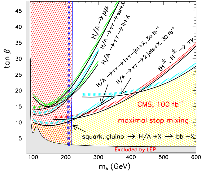
Figure 37: The 5\sigma discovery contours for MSSM Higgs bosons in the (m_A, \tan\beta) -plane for an integrated luminosity of 100 \text{ fb}^{-1} for the SUSY parameter point with m_{\tilde{g}} = 1200 \text{ GeV}/c^2 , m_{\tilde{q}} = 800 \text{ GeV}/c^2 , M_2 = 350 \text{ GeV}/c^2 and \mu = 150 \text{ GeV}/c^2 . In the region with m_A < 220 \text{ GeV}/c^2 the heavier Higgs bosons H and A can be detected in cascade decays of squarks and gluinos (from Ref. 156).
