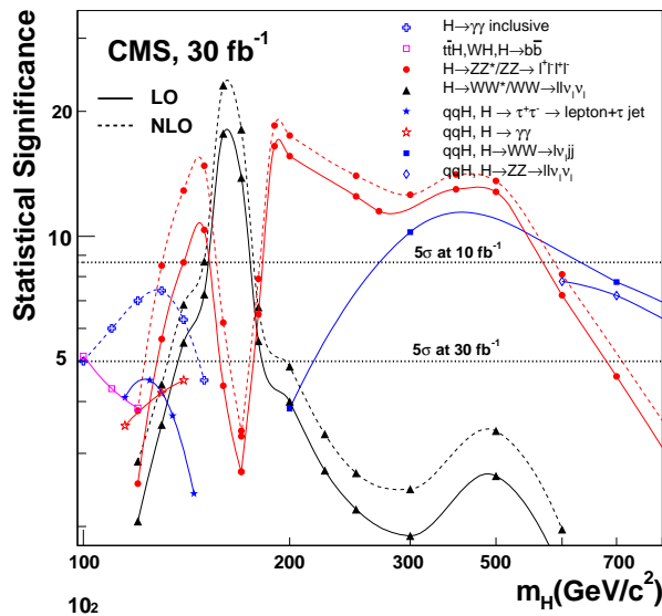
Figure 25: CMS sensitivity for the discovery of a Standard Model Higgs boson for an integrated luminosity of 30 \text{ fb}^{-1} over the full mass region. The signal significances are plotted for individual channels, as well as for the combination of channels. A systematic uncertainty of \pm 5\% on the background has been included for the H \rightarrow WW^{(*)} \rightarrow \ell\nu \ell\nu channel. For the channels H \rightarrow \gamma\gamma , H \rightarrow ZZ^{(*)} \rightarrow 4\ell and H \rightarrow WW^{(*)} \rightarrow \ell\nu \ell\nu results are shown for both leading order and next-to-leading order predictions for signals and backgrounds (from Ref. 69).
