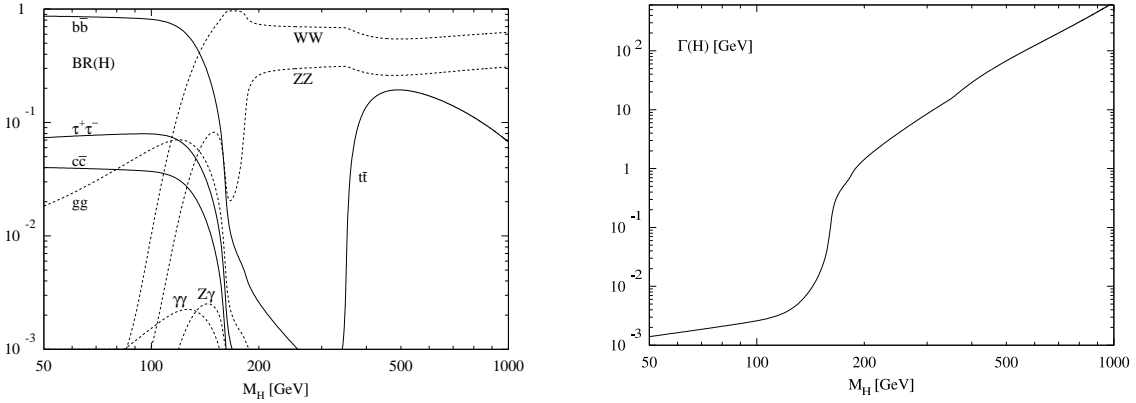
Figure 5: Branching fractions (left) and total decay width (right) of the Standard Model Higgs boson as a function of Higgs boson mass (from Ref. 42).
