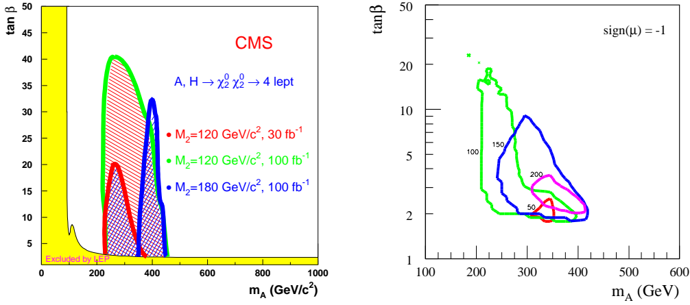
Figure 34: (Left) The 5 \sigma discovery contours in the (m_A, \tan\beta) -plane for H/A \rightarrow \chi_2^0 \chi_2^0 \rightarrow \chi_1^0 \ell\ell \chi_1^0 \ell\ell decays for different SUSY parameters and integrated luminosities (from Ref. 69). (Right) The 5 \sigma discovery contours in the (m_A, \tan\beta) -plane for H/A \rightarrow \chi_2^0 \chi_2^0 \rightarrow \chi_1^0 \ell\ell \chi_1^0 \ell\ell in the mSUGRA scenario for fixed m_0 = 50, 100 and 200 \text{ GeV}/c^2 , A_0 = 0 and \mu < 0 . The parameter m_{1/2} has been scanned in the range between 100 and 300 \text{ GeV}/c^2 . An integrated luminosity of 300 \text{ fb}^{-1} is assumed (from Ref. 68).
