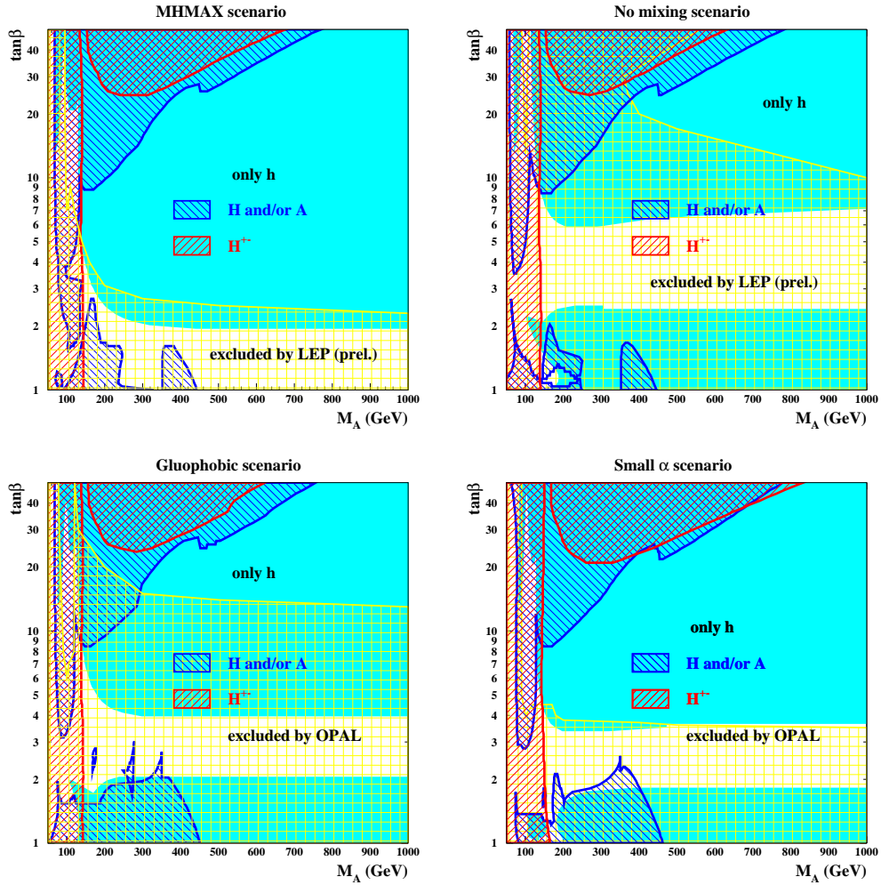
Figure 32: The overall 5\sigma discovery potential for MSSM Higgs bosons at the LHC for an integrated luminosity of 30\text{fb}^{-1} in the four benchmark scenarios (see text). In the shaded area (cyan) only the light CP-even Higgs boson h can be observed. In the blue left-hatched area the heavy neutral Higgs bosons H and/or A , and in the red right-hatched area the charged Higgs bosons H^\pm can be detected. The cross hatched yellow region is excluded by searches at LEP (from Ref. 148).
