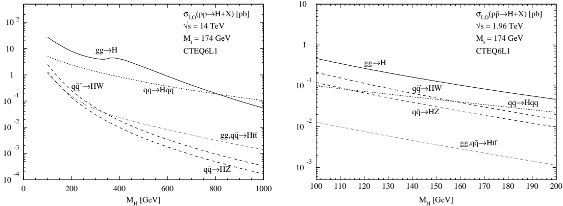
Figure 1: Leading order production cross sections for a Standard Model Higgs boson as a function of the Higgs boson mass at the LHC 14 TeV pp collider (left) and at the 1.96 TeV Tevatron p\bar{p} collider (right). In the cross section calculation the CTEQ6L1 structure function parametrization has been used. (The calculations have been performed by M. Spira, Ref. 19)
