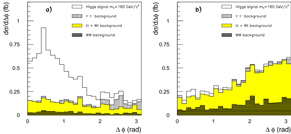
Figure 20: Distributions of the azimuthal opening angle \Delta\phi between the two leptons for events in the signal region ( M_T < 175 \text{ GeV}/c^2 ) (left) and events outside the signal region ( M_T > 175 \text{ GeV}/c^2 ) (right). The accepted cross sections d\sigma/d\Delta\phi (in \text{fb}/0.13 \text{ rad} ) including all efficiency and acceptance factors are shown in both cases (from Ref. 79).
