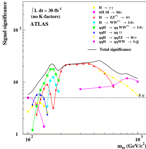
Figure 24: ATLAS sensitivity for the discovery of a Standard Model Higgs boson for an integrated luminosity of 30 \text{ fb}^{-1} over the full mass region. The signal significances are plotted for individual channels, as well as for the combination of channels. Systematic uncertainties on the background have been included for the vector boson fusion channels ( \pm 10\% ) and for the H \rightarrow WW^{(*)} \rightarrow \ell\nu \ell\nu channel ( \pm 5\% ).
