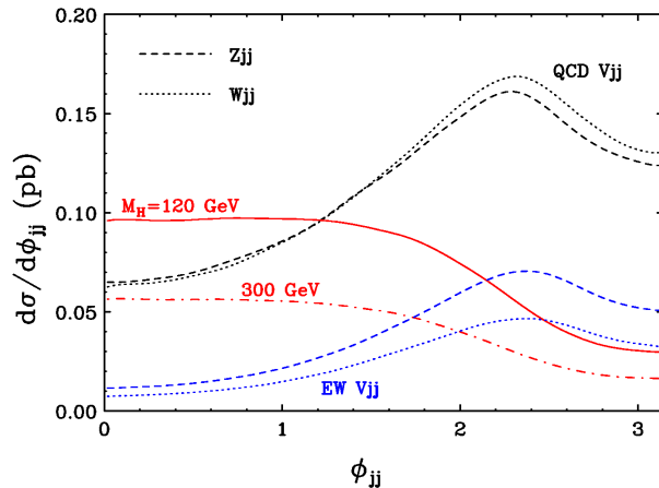
Figure 39: Distribution of the azimuthal angle separation ( \phi_{jj} ) between the two tagging jets for the Wjj and Zjj backgrounds from QCD and electroweak production and Higgs boson signals with m_H = 120 and 300 \text{ GeV}/c^2 . Results are shown after applying the jet tag requirements and the cut \cancel{E}_T > 100 \text{ GeV} (from Ref. 175).
