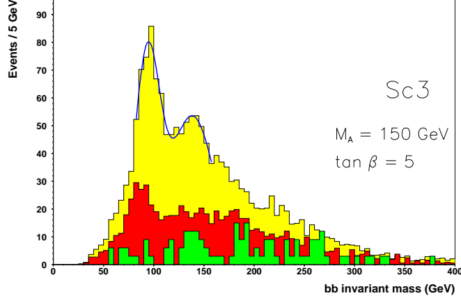
Figure 36: The reconstructed b\bar{b} invariant mass spectrum for a SUSY scenario with M_2 = 350 \text{ GeV}/c^2 , \mu = 150 \text{ GeV}/c^2 , m_{\tilde{g}} = 1200 \text{ GeV}/c^2 and m_{\tilde{q}} = 800 \text{ GeV}/c^2 in a simulation of the CMS experiment, assuming an integrated luminosity of 30 \text{ fb}^{-1} . The two mass peaks result from decays of the lighter h and the heavier H/A Higgs bosons. They are shown on top of the backgrounds from SUSY processes (dark) and from Standard Model t\bar{t} production (light) (from Ref. 156).
