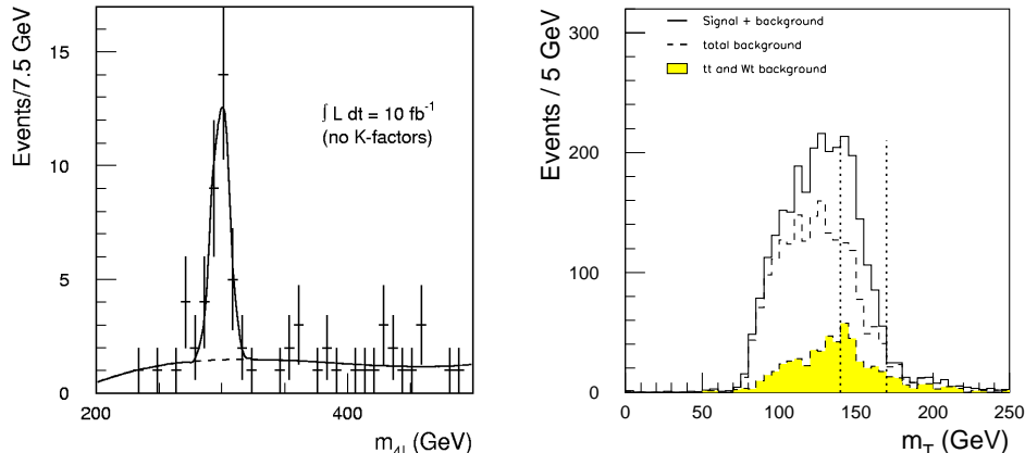
Figure 16: (Left) Expected H \rightarrow ZZ \rightarrow 4\ell signal above the background for m_H = 300 \text{ GeV}/c^2 and for an integrated luminosity of 10 \text{ fb}^{-1} in the ATLAS experiment (from Ref. 68). (Right) Transverse mass distribution for the summed H \rightarrow WW^* \rightarrow \ell\nu \ell\nu signal ( m_H = 150 \text{ GeV}/c^2 ) and total background, for an integrated luminosity of 30 \text{ fb}^{-1} . The distribution for the background alone is also shown separately. The shaded histogram represents the contributions from the Wt and t\bar{t} backgrounds. The dashed lines indicate the selected signal region (from Ref. 68).
