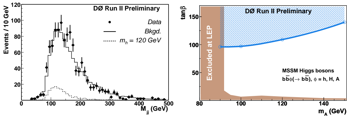
Figure 11: (Left) Invariant mass spectrum of the two leading jets in the 3-jet sample with three b -tags after final cuts in the DØ search for bh production using Run II data corresponding to an integrated luminosity of 131 \text{ pb}^{-1} ; the dashed histogram shows the distribution for a Higgs signal with m_H = 120 \text{ GeV}/c^2 and \tan\beta=100 ; (Right) Regions in (m_A, \tan\beta) excluded by this analysis at 95% C.L. in comparison with LEP limits (from Ref. 59).
