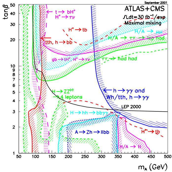
Figure 29: The combined sensitivity of the ATLAS and CMS experiments for the discovery of MSSM Higgs bosons in the maximal mixing scenario for an integrated luminosity of 30 \text{ fb}^{-1} . The 5\sigma discovery contour curves are shown in the (m_A, \tan\beta) -plane for individual channels not including the vector boson fusion channels. The limit from the LEP experiments is superimposed (from Ref. 133).
