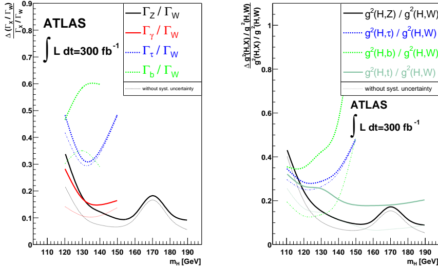
Figure 26: The expected relative errors for the measurement of relative branching ratios (left) and relative couplings (right), normalized to those of the H \rightarrow WW decay and assuming an integrated luminosity of 300 \text{ fb}^{-1} for one experiment. The dashed lines give the expected relative error without systematic uncertainties (from Ref. 111).
