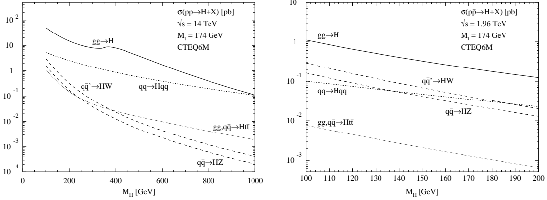
Figure 4: NLO production cross sections for a Standard Model Higgs boson as a function of the Higgs boson mass at the LHC 14 TeV pp collider (left) and at the 1.96 TeV Tevatron p\bar{p} collider (right). In the cross section calculation the CTEQ6M structure function parametrization has been used. (The calculations have been performed by M. Spira, Ref. 19)
