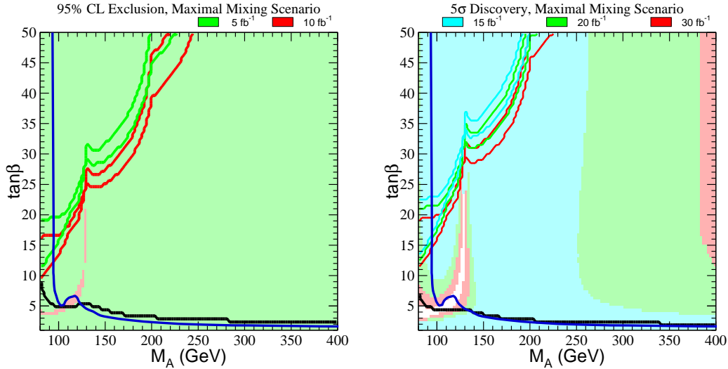
Figure 13: Luminosity required for exclusion at 95% C.L. (left) or 5\sigma discovery (right) of a SUSY Higgs boson as a function of m_A and \tan\beta within the m_h -max scenario (taken from Ref. 36 and modified to include the most recent LEP2 limit 13 ). Shaded regions indicate the reach of WH and ZH searches, the region above the diagonal lines are accessible to searches for \Phi b(b) , the dark line indicates the LEP2 limit.
