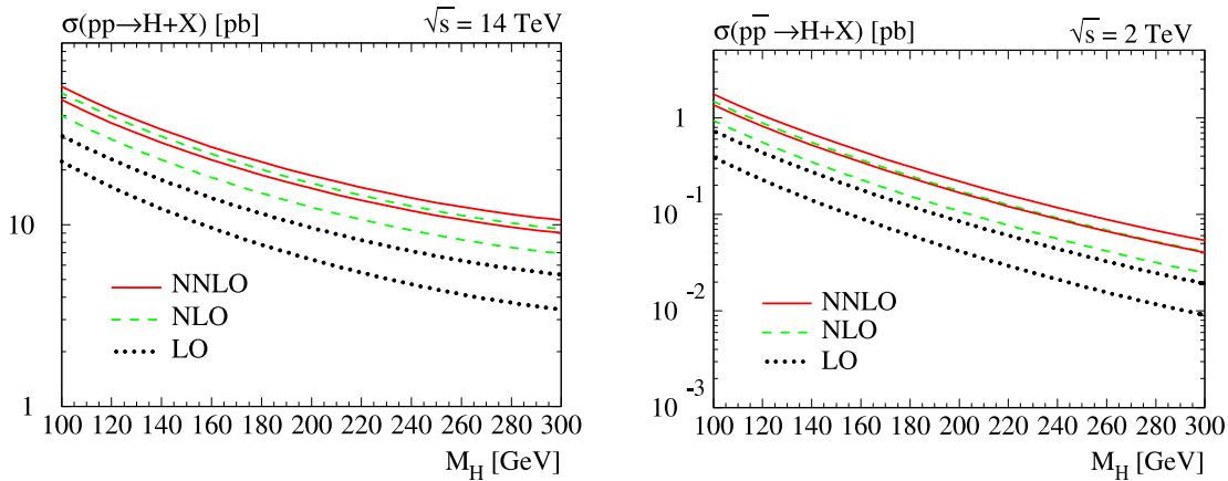
Figure 2: Gluon-fusion production cross section for a Standard Model Higgs boson at the LHC 14 TeV pp collider (left) and at the Tevatron 2 TeV p\bar{p} collider (right) at leading (dotted), next-to-leading (dashed) and next-to-next-to-leading order (solid). The upper (lower) curve of each pair corresponds to a choice of the renormalization and factorization scale of \mu_R = \mu_F = m_H/2 ( \mu_R = \mu_F = 2 m_H ) (from Ref. 26, see also Refs. 22, 23, 24).
