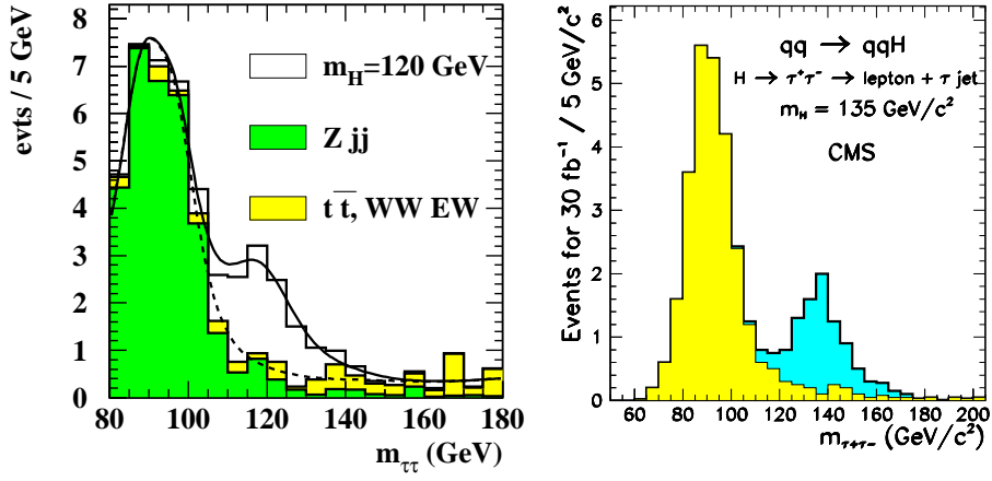
Figure 21: (Left) The reconstructed \tau\tau invariant mass for a Higgs boson signal of 120 \text{ GeV}/c^2 in the e\mu channel above all backgrounds after application of all cuts except the mass window cut around the Higgs boson mass. The number of signal and background events are shown for an integrated luminosity of 30 \text{ fb}^{-1} (from Ref. 79). (Right) The same, for the l -had channel and for a Higgs boson with m_H = 135 \text{ GeV}/c^2 (from Ref. 69).
