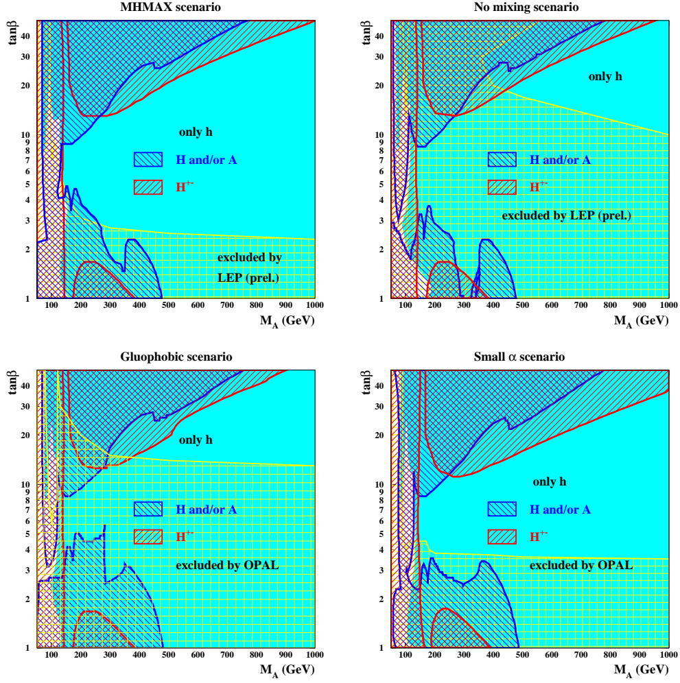
Figure 33: The same as Fig. 32, but for an integrated luminosity of 300\text{fb}^{-1} (except for the A/H \rightarrow \tau\tau decay mode, for which an integrated luminosity of 30\text{fb}^{-1} has been assumed) (from Ref. 148).
