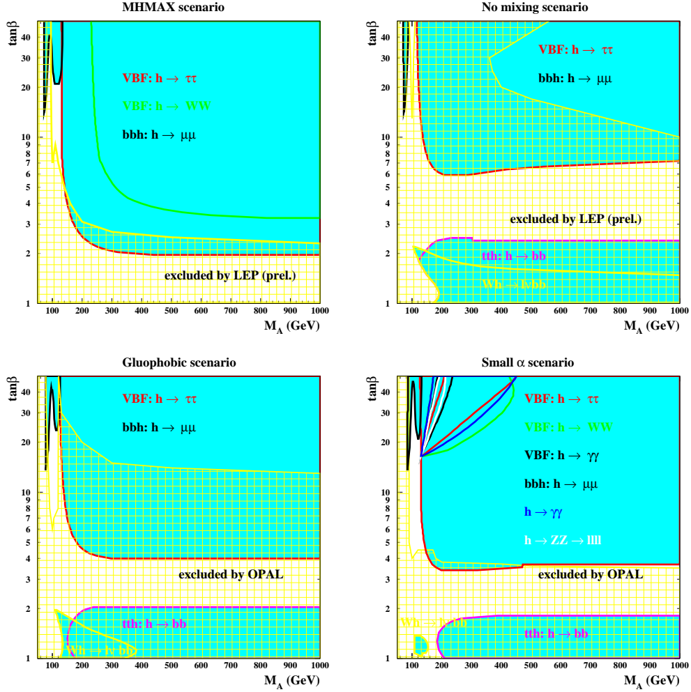
Figure 31: The 5\sigma discovery contours for the light CP even Higgs boson h in the (m_A, \tan\beta) -plane after collecting 30\text{fb}^{-1} in the ATLAS experiment for the four benchmark scenarios considered: the m_h -max scenario, the no mixing scenario, the gluophobic and small \alpha scenario (see text for details). The cross-hatched yellow region is excluded by searches at LEP (from Ref. 148).
