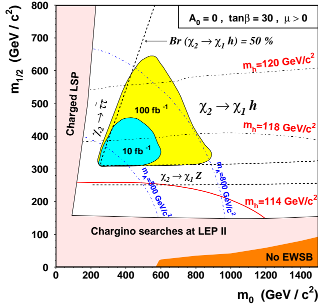
Figure 35: The 5\sigma discovery contours in the (m_0, m_{1/2}) -plane for the CP-even Higgs bosons h via the decay h \rightarrow b\bar{b} from \chi_2^0 \rightarrow \chi_1^0 h decays in squark and gluino cascades for mSUGRA scenarios with \tan\beta = 30 , A_0 = 0 and \mu > 0 for 10 and 100 \text{ fb}^{-1} . The regions excluded by experimental and theoretical constraints are indicated as well (from Ref. 69).
