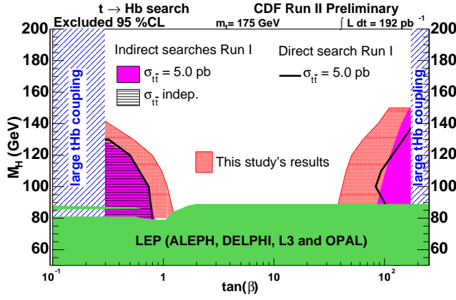
Figure 14: Regions in the MSSM (m_{H^\pm}, \tan\beta) -plane excluded by the CDF Run II t\bar{t} cross section measurements, in comparison with regions excluded at LEP and Run I; Tevatron results do not apply for non-perturbative Ht\bar{b} couplings at small and large \tan\beta (from Ref. 64).
