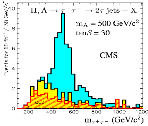
Figure 28: The reconstructed \tau\tau invariant mass distribution in the fully hadronic final state ( \tau_{had} - \tau_{had} ) from the process gg \rightarrow b\bar{b} H/A \rightarrow b\bar{b} \tau\tau . The H/A signal (dark) for m_A = 500 \text{ GeV}/c^2 and \tan\beta=30 is shown on top of the background for an integrated luminosity of 60 \text{ fb}^{-1} (from Ref. 69).
