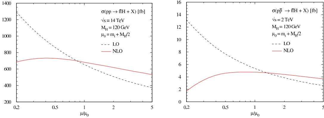
Figure 3: Variation of the t\bar{t}H production cross section at the LHC 14 TeV pp collider (left) and at the Tevatron 2 TeV p\bar{p} collider (right) with the renormalization and factorization scale \mu = \mu_R = \mu_F , varied around the value \mu_0 = m_t + m_H/2 (from Refs. 27 and 28).
