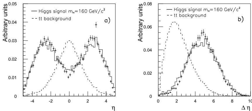
Figure 17: (Left) Pseudorapidity distribution of the tag jets in signal events with m_H = 160 \text{ GeV}/c^2 and for t\bar{t} background events. (Right) Separation \Delta\eta between the tag jets for the same types of events. The full histograms show the distributions at parton level, the dots represent the distributions at reconstruction level, after the tagging algorithm has been applied. The corresponding distributions for jets identified as tag jets in t\bar{t} events are superimposed as dashed histograms. All distributions are normalized to unity (from Ref. 79).
