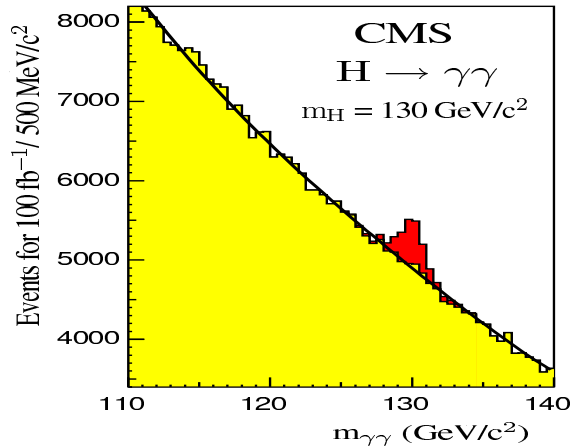
Figure 15: Reconstructed \gamma\gamma invariant mass distribution of a H \rightarrow \gamma\gamma signal (dark) with m_H = 130 \text{ GeV}/c^2 and the background (light) for an integrated luminosity of 100 \text{ fb}^{-1} in the CMS experiment (from Ref. 69).
