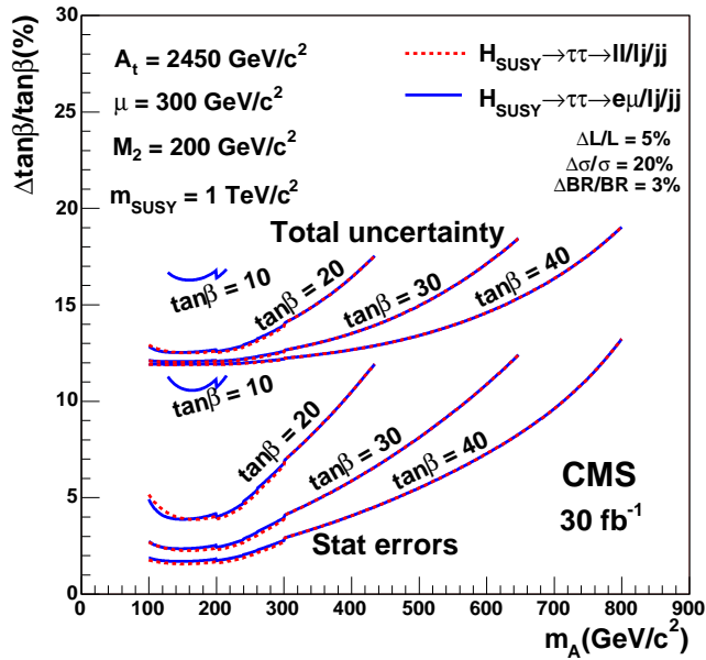
Figure 38: Relative uncertainty on the \tan\beta measurement in the CMS experiment assuming an integrated luminosity of 30 \text{ fb}^{-1} . The uncertainty is given for fixed values of \tan\beta as a function of m_A including statistical (lower curves) and statistical plus systematic uncertainties (upper curves) (from Ref. 161).
