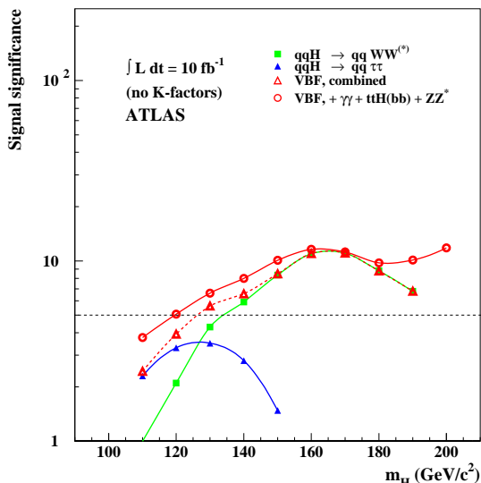
Figure 22: ATLAS sensitivity for the discovery of a Standard Model Higgs boson for an integrated luminosity of 10 \text{ fb}^{-1} in the low mass region. The signal significances are plotted for individual channels, as well as for the combination of several channels. A systematic uncertainty of \pm 10\% on the background has been included for the vector boson fusion channels (from Ref. 79).
