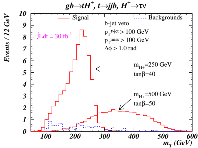
Figure 30: The reconstructed transverse mass of the \tau_{had} - \cancel{P}_T system from the process gb \rightarrow H^+ t \rightarrow \tau\nu qqb for charged Higgs bosons with masses of 250 GeV/c 2 (at \tan\beta = 40 ) and 500 GeV/c 2 (at \tan\beta = 50 ) in comparison to the background. The simulation has been performed for the ATLAS experiment assuming an integrated luminosity of 30 fb -1 (from Ref. 141).
