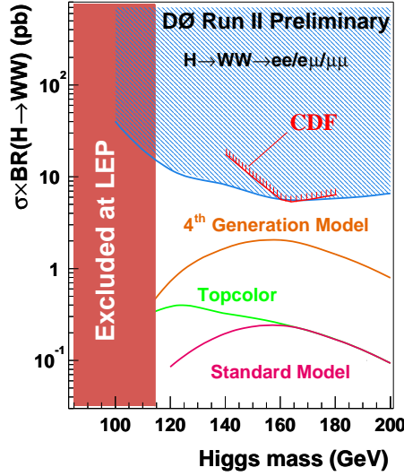
Figure 10: Upper limit (at 95% C.L.) on the cross section \sigma \cdot BR(H \rightarrow WW) set by the D\phi Collaboration using Run II data corresponding to an integrated luminosity of 176 \text{ pb}^{-1} , with the limit set by the CDF Collaboration ( 184 \text{ pb}^{-1} ) superimposed (from Ref. 52). The limits are compared to expectations from Standard Model Higgs production and alternative models.
