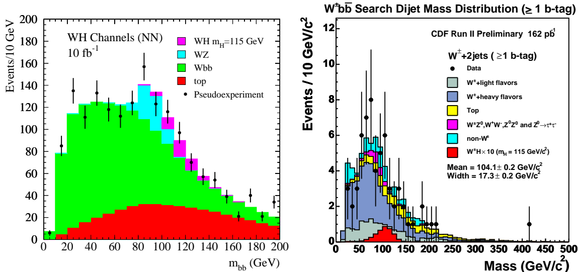
Figure 7: Invariant b\bar{b} mass spectrum in search for WH production in full simulation of Tevatron data corresponding to an integrated luminosity of 10 \text{ fb}^{-1} (left, from Ref. 49) and in CDF Run II data corresponding to an integrated luminosity of 162 \text{ pb}^{-1} in comparison with signal and background expectation (right, from Ref. 51).
