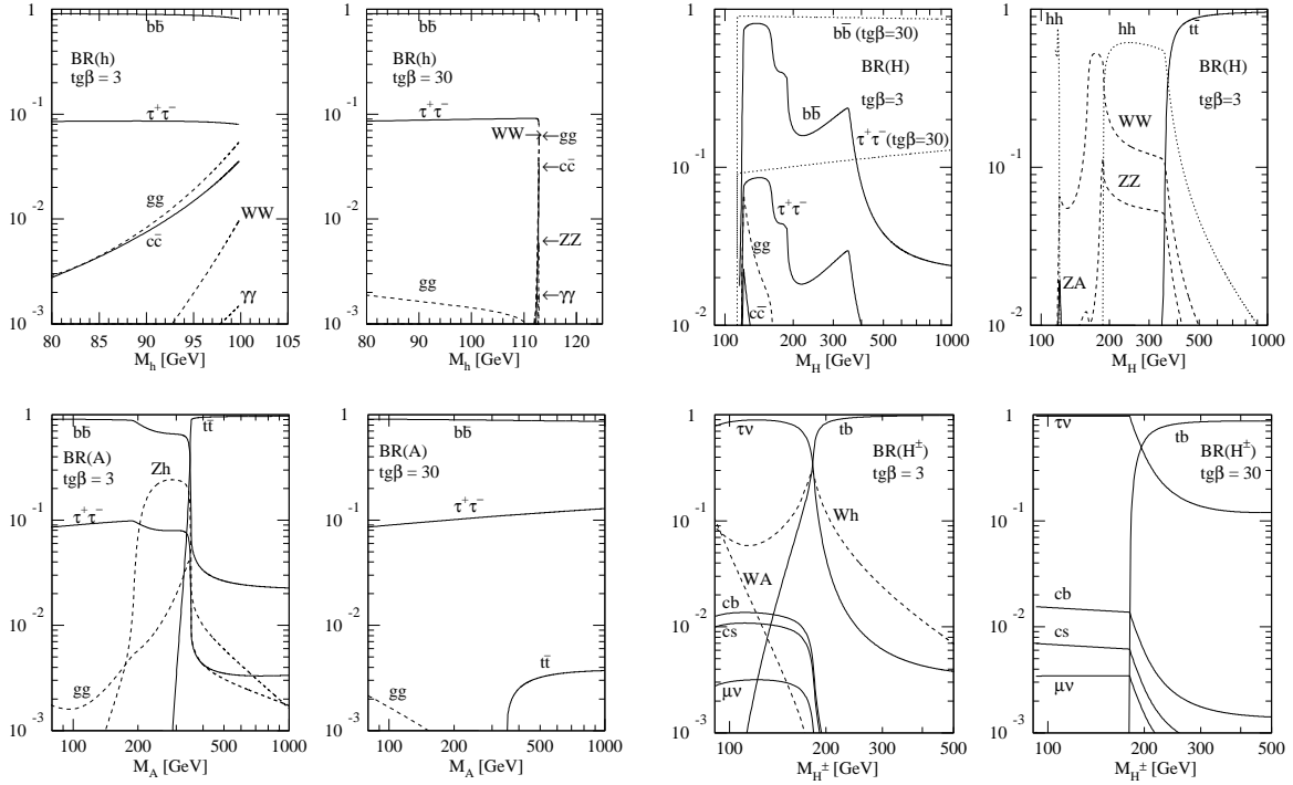
Figure 6: Branching fractions of the MSSM Higgs bosons as a function of their masses for \tan\beta=3 and \tan\beta=30 assuming a SUSY mass scale of 1 \text{ TeV}/c^2 and vanishing mixing (from Ref. 42).
