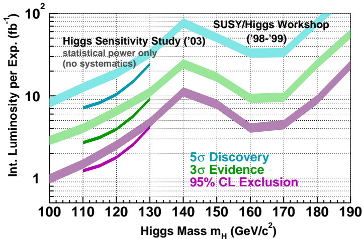
Figure 8: The integrated luminosity required per experiment for a 95% C.L. exclusion, a 3\sigma and a 5\sigma discovery of a Standard Model Higgs boson at the Tevatron as a function of the Higgs boson mass. Thin lines show recent estimates based on full simulation verified with Run II data 49 for the combination of searches for associated production with a vector boson with no systematic uncertainties included. Thick lines indicate results of an earlier study 36 with fast simulation which includes the combination with searches for gg \rightarrow H \rightarrow WW (see Section 4.2). For the latter, the line thickness indicates the impact of systematic uncertainties.
